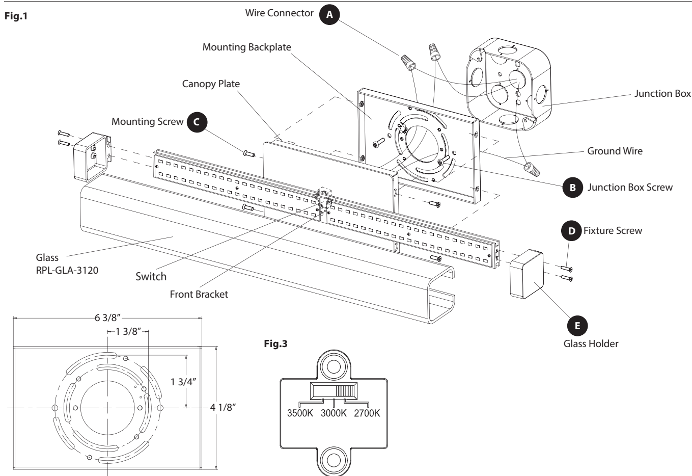
WS-3120 Back Plate Dimensions
