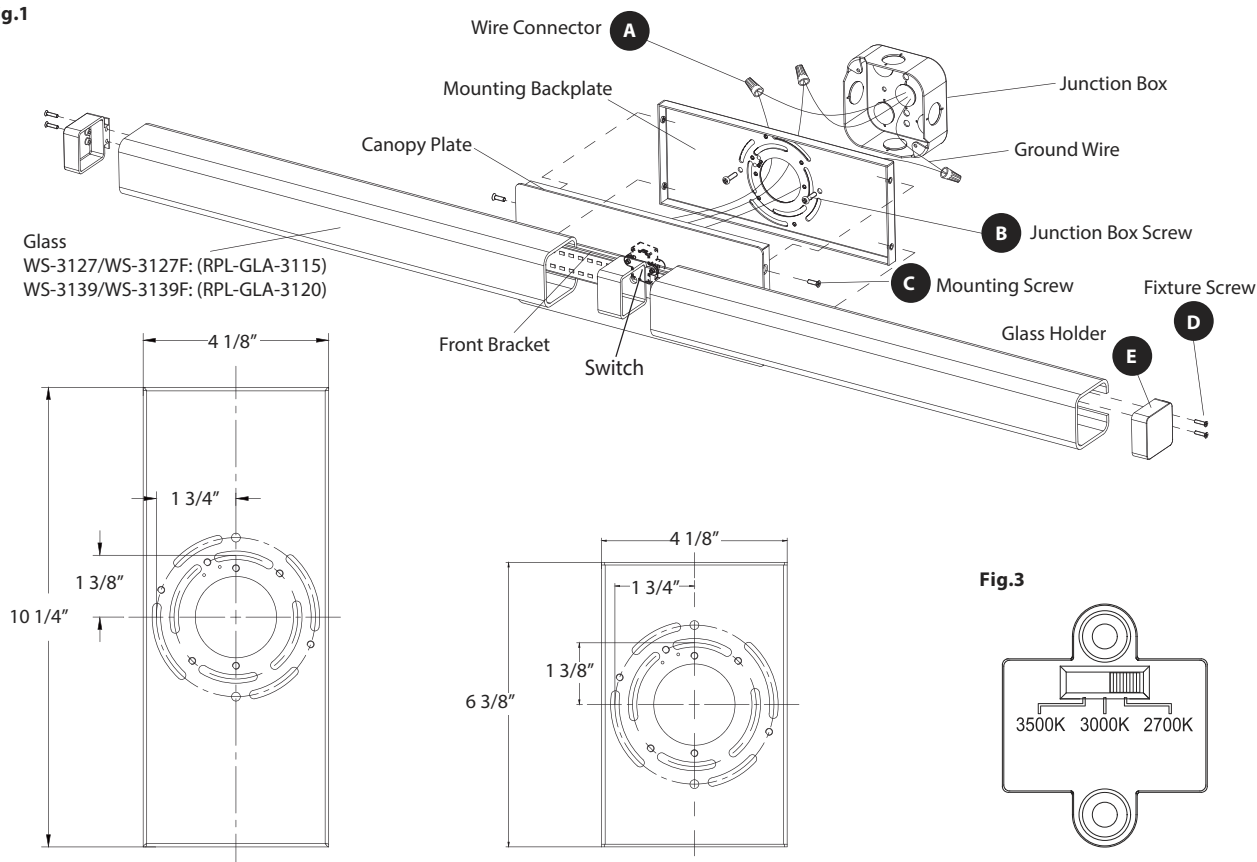
WS-3139/WS-3139F Back Plate Dimensions
