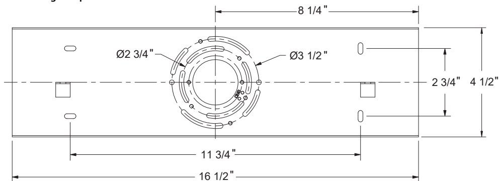
Mounting Backplate Dimensions
